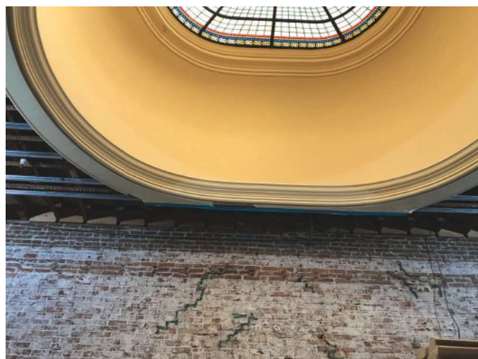
Fig. 2: The unreinforced masonry walls crumbled while the glass from the vaulted glass dome on the second floor was undamaged
